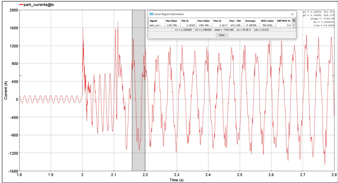
Figure 10 Time-domain verification of SSCI condition
