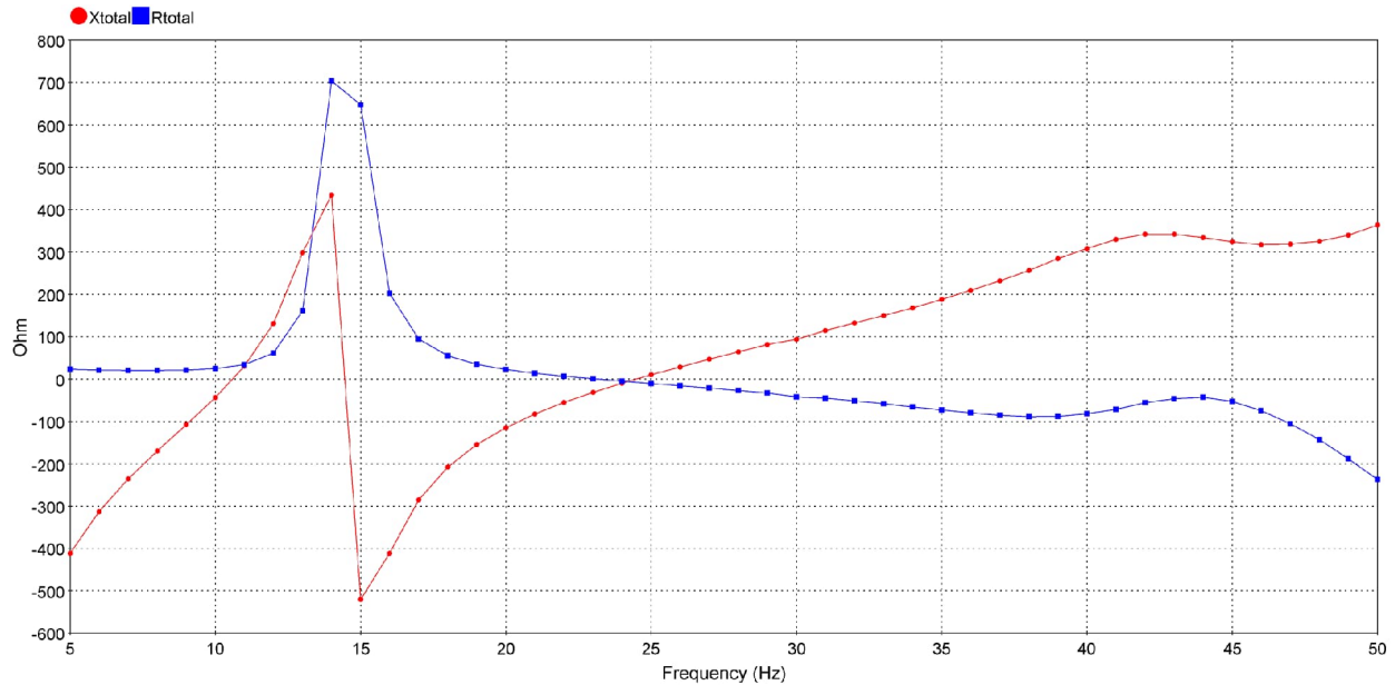
Figure 9 Combined scan: WP impedance added to Grid impedance
