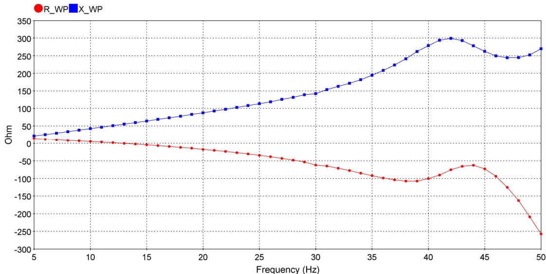
Figure 8 WP impedance scan using “Input Impedance TD”
