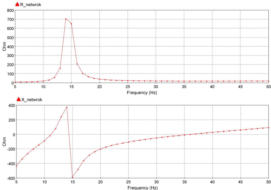
Figure 6 Grid side scan, R and X parts of impedance seen from ZIN1 in Figure 5
