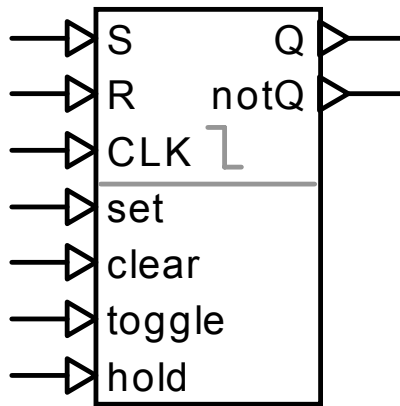
S-R flip-flop nor-gated
